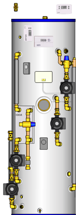
The GX Heat Bank with fitted Solar Controls Patented DPS Technology
